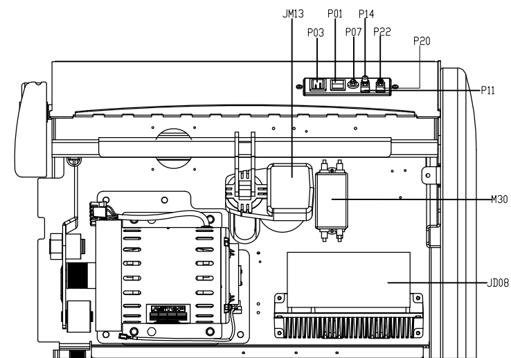
Top View of Electrical Components
